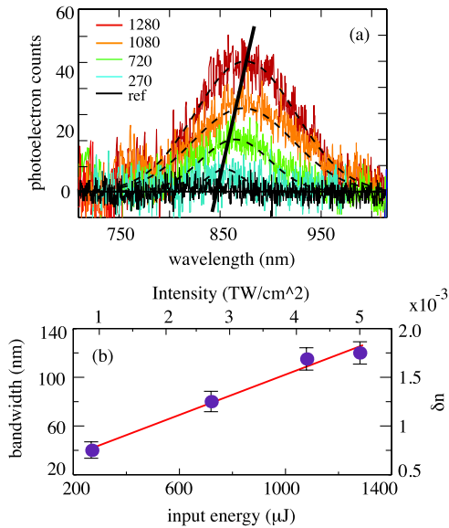
FIG. 3 (color online). (a) Spectra generated by a Bessel filament. Five different curves are shown corresponding to a reference spectrum obtained with a Gaussian pulse (black line) and indicated Bessel energies (in \mu\text{J} ). Dashed lines are guides for the eye. The solid line connects the spectral peaks, highlighting the \sim 40 nm shift with increasing energy, in close agreement with the predicted 45 nm shift. (b) Bandwidths at FWHM and RIP \delta n versus input energy and intensity. Solid line: linear fit \delta n = n_2 I with n_2 = 2.8 \times 10^{-16} \text{ cm}^2/\text{W} .
