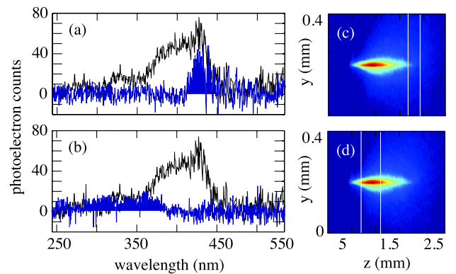
FIG. 4 (color online). Spectra generated by the spontaneous filament. (a)–(b) shaded areas: spectra measured for two different positions of the imaging spectrometer input slit. The light gray curves in both figures show the spectrum measured with the input slit fully open. The filament, imaged from the side at 90^\circ , is shown in (c) and (d). The vertical white lines show the position of the input slit.
