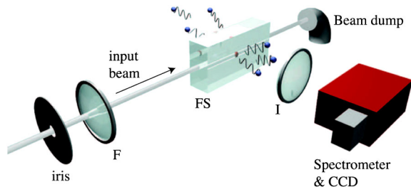
FIG. 1 (color online). Experimental layout used for detecting analogue Hawking radiation. The input laser pulse is focused into a sample of fused silica (FS) using an axicon or lens ( F ). An imaging lens ( I ) collects the photons emitted at 90^\circ and sends them to an imaging spectrometer coupled to a cooled CCD camera.
