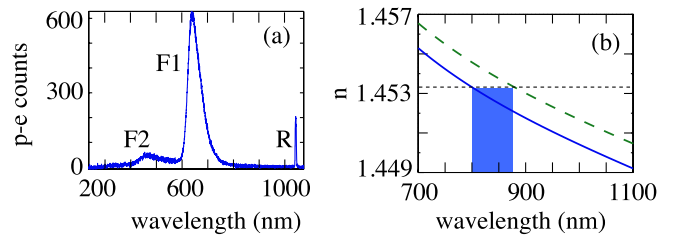
FIG. 2 (color online). (a) Measured CCD photo-electron ( p - e ) counts generated by the fused silica fluorescence spectrum. (b) Prediction of the Hawking emission spectral range for the case of fused silica: n_0 (blue solid line) and n_0 + \delta n (green dashed line) with \delta n = 0.001 . The shaded area indicates the spectral emission region predicted for a Bessel filament.
