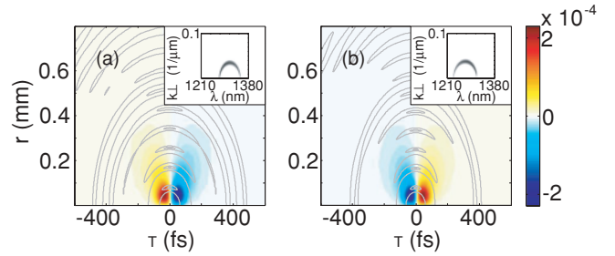
FIG. 6. (Color online) Transverse flux J_r for stationary CWP of the O-wave type for different propagation velocities of the envelope peak. (a) V = 0.9995 V_G ; (b) V = 1.0005 V_G . The gray contour plots show the intensity over four decades. The insets show the corresponding spectral \lambda , k_\perp features. Color scale in arbitrary units.
