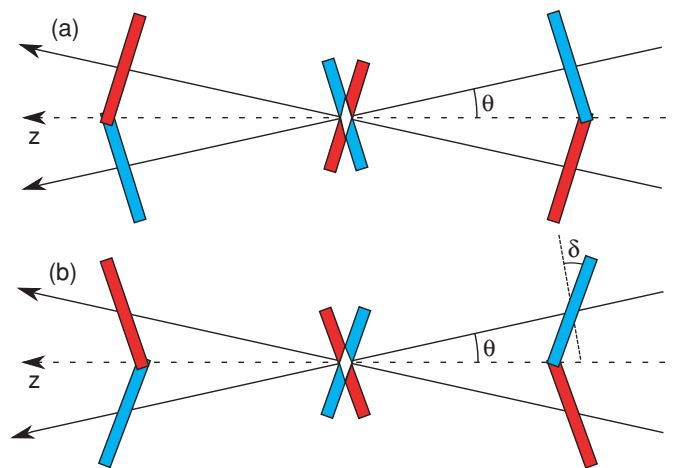
FIG. 4. (Color online) Simple representation of the propagation of the expected transverse flux for the propagation of (a) a BXP and (b) a rotationally symmetric tilted pulse. The red (blue) color corresponds to flux directed upward (downward) with respect to the vertical axis.
